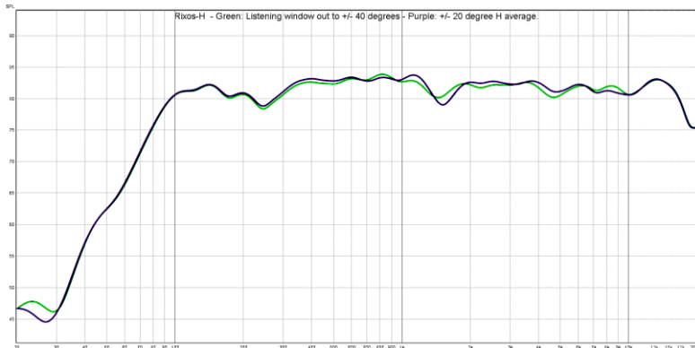
Responses: Listening Window and +/-20 H* *Most H speakers have a real problem here!
